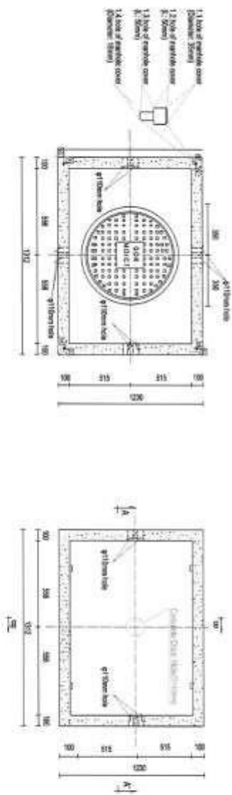
CONCRETE REINFORCEMENT MANHOLE (Figure 15)
